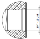
DETAIL A SCALE 2 : 1 INLET & OUTLET GAS SEAT ACCORDING TO SAE J1926
