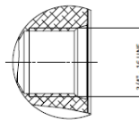
DETAIL A SCALE 2 : 1 INLET & OUTLET GAS SEAT ACCORDING TO SAE J1926
